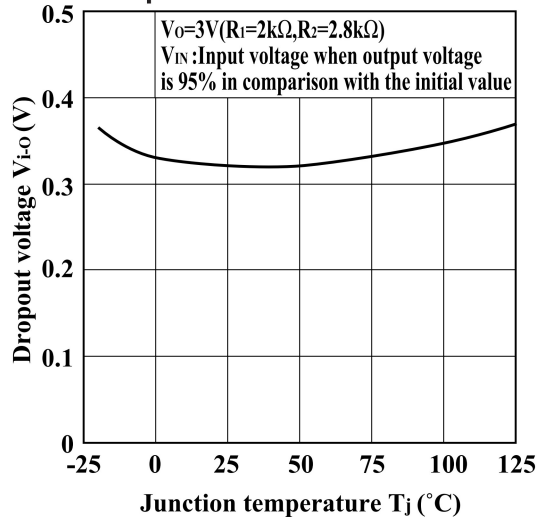
Fig.9 Dropout Voltage vs. Junction Temperature
