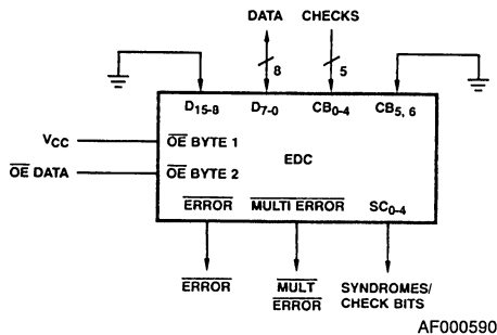
Figure 17. 8-Bit Configuration
