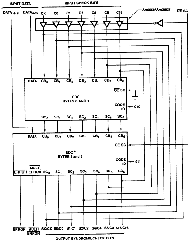
Figure 8. 32-Bit Configuration
