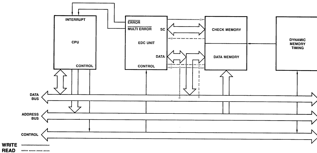
Figure 11. Check-Only Configuration
