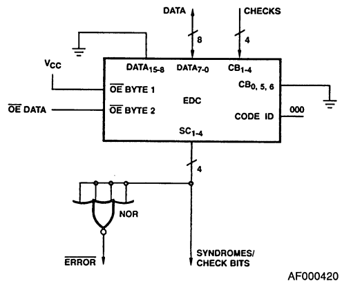
Figure 19. 8-Bit Single Error Correction Only
