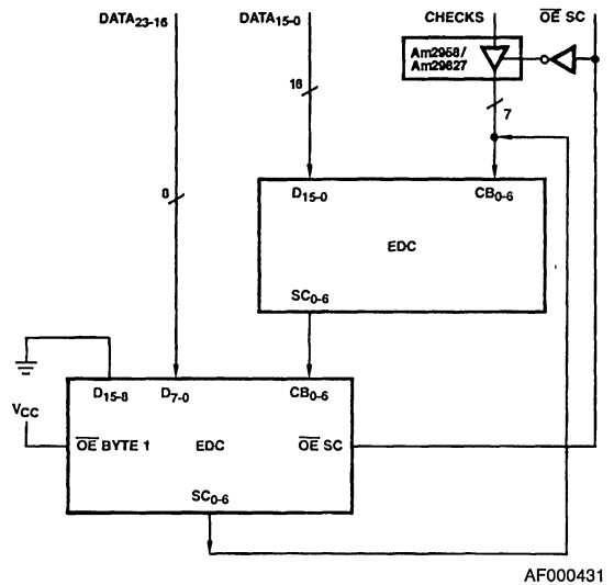
Figure 18. 24-Bit Configuration
