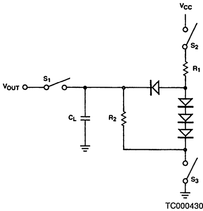
Figure 24. Three-State Outputs
