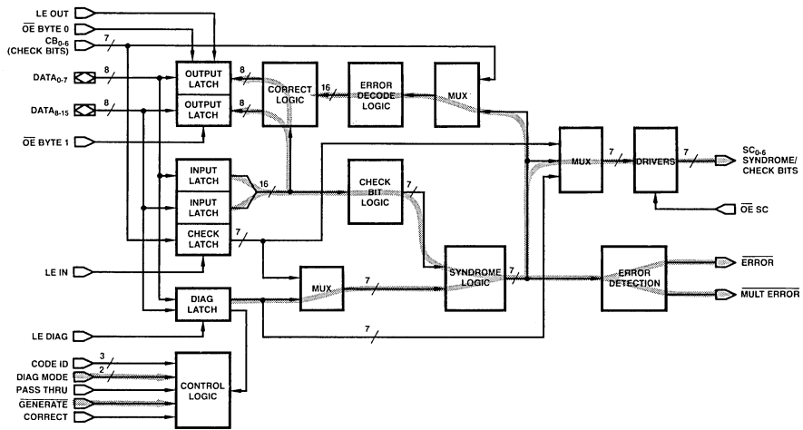
Figure 4. Diagnostic Detect and Correct Data Path
