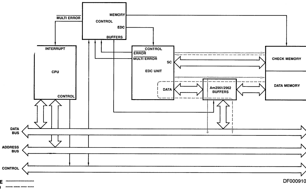
Figure 12. Correct-Always Configuration
